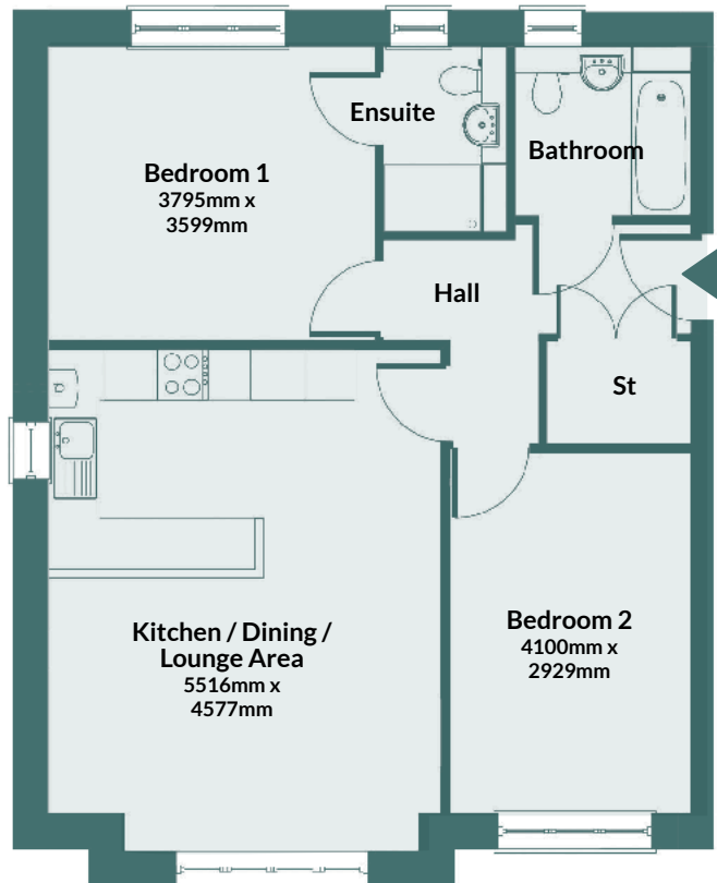
UNIT TYPE 3
