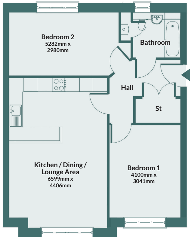
UNIT TYPE 4
